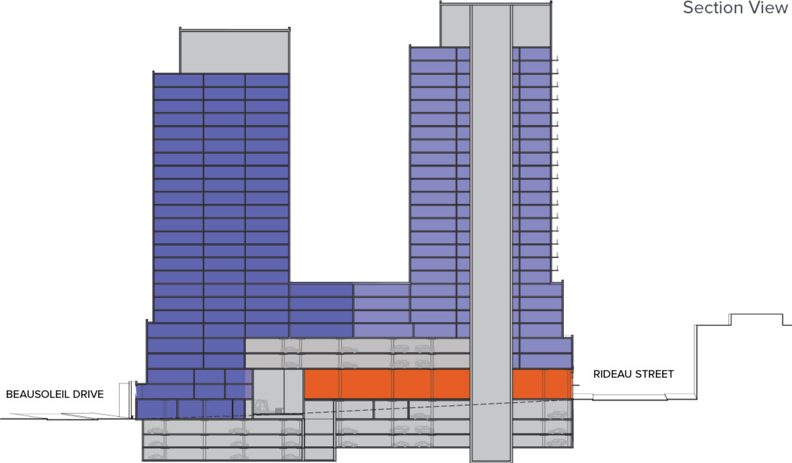
Section View
